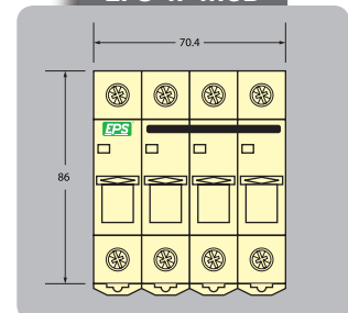
EPS 4P MCB
