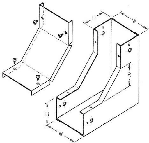
90 DEG. VERTICAL INSIDRISER
