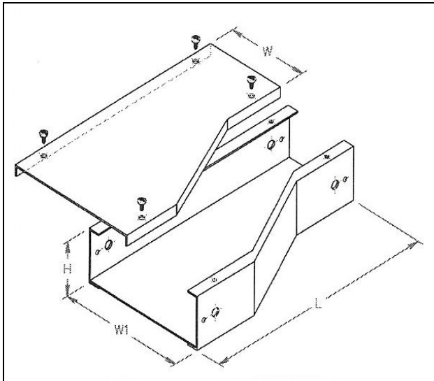
LEFT-HAND REDUCER
