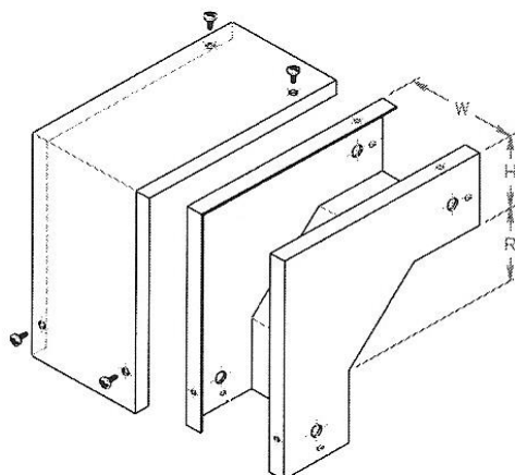
90 DEG. VERTICAL INSIDRISER
