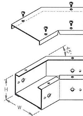
45 DEG. HORIZONTAL FLAT ELBOW
