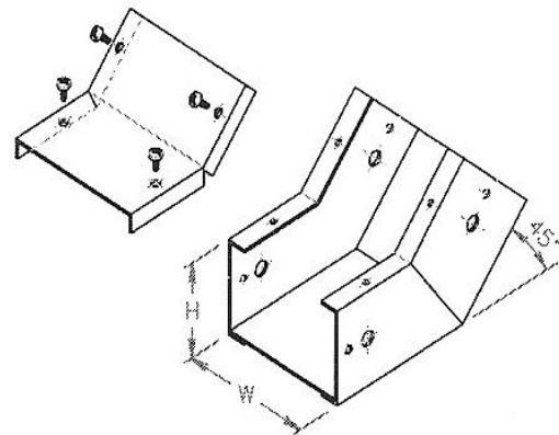
45 DEG. VERTICAL INSIDRISER
