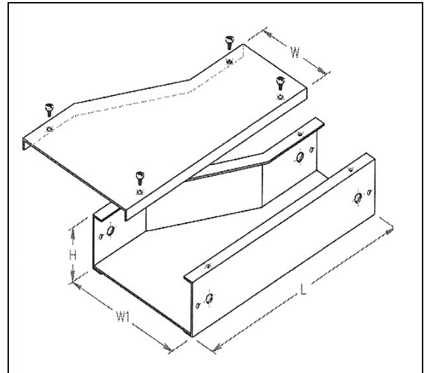
RIGHT-HAND REDUCER
