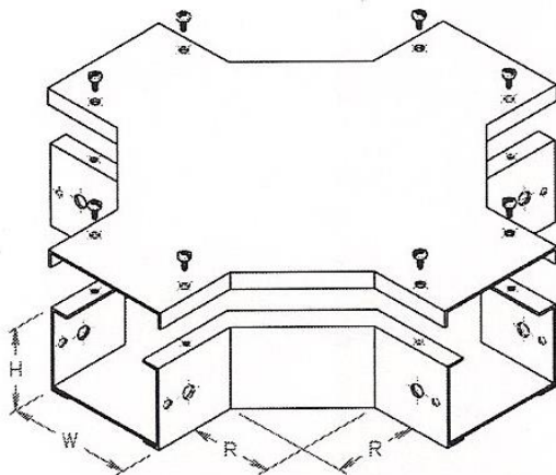
HORIZONTAL EQUAL CROSS
