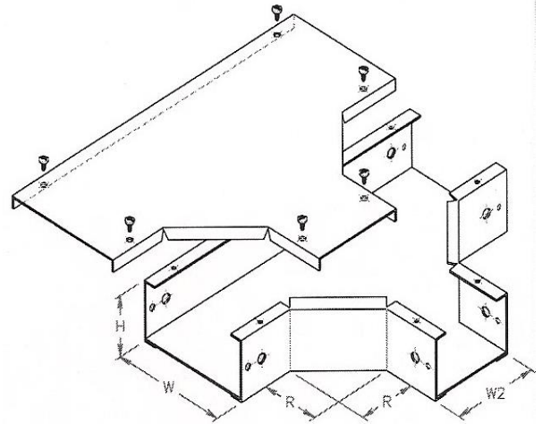
HORIZONTAL UNEQUAL TEE
