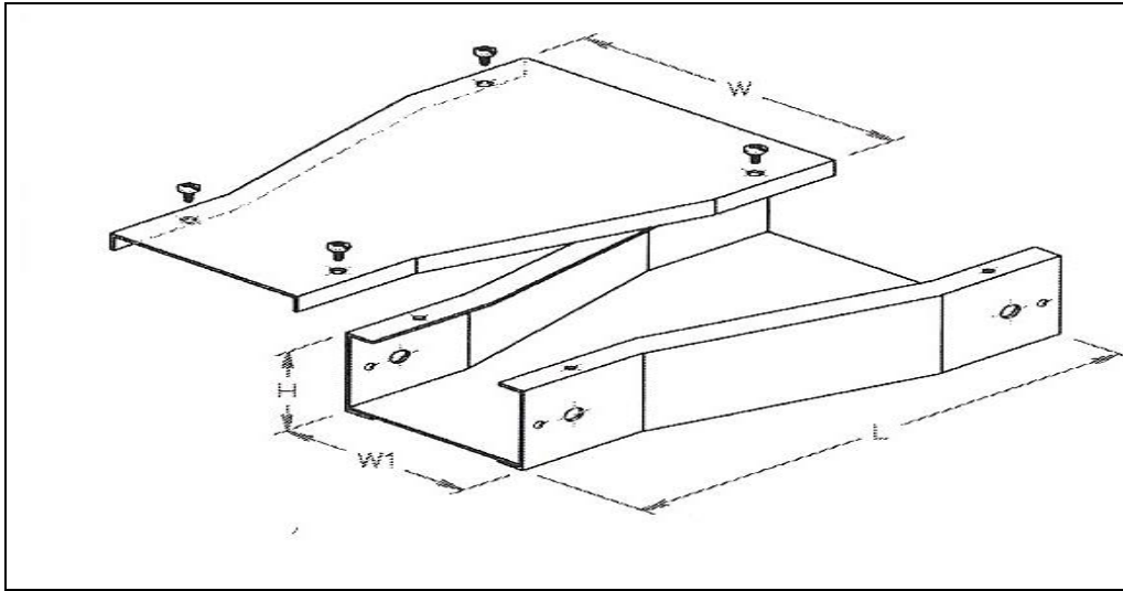
STRAIGHT REDUCER
