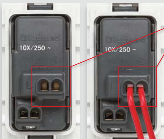
Wires are held in place with the clamping plate. This reduces the risk of damaging wires. The combination of double entry and clamping plate ensures long term reliability of the connection.
