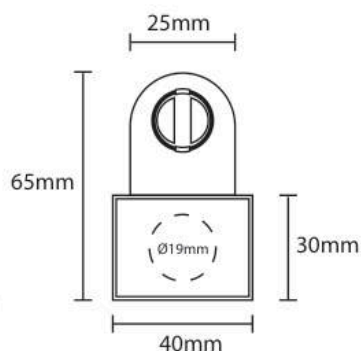
Thick Casing (Single Tube)
