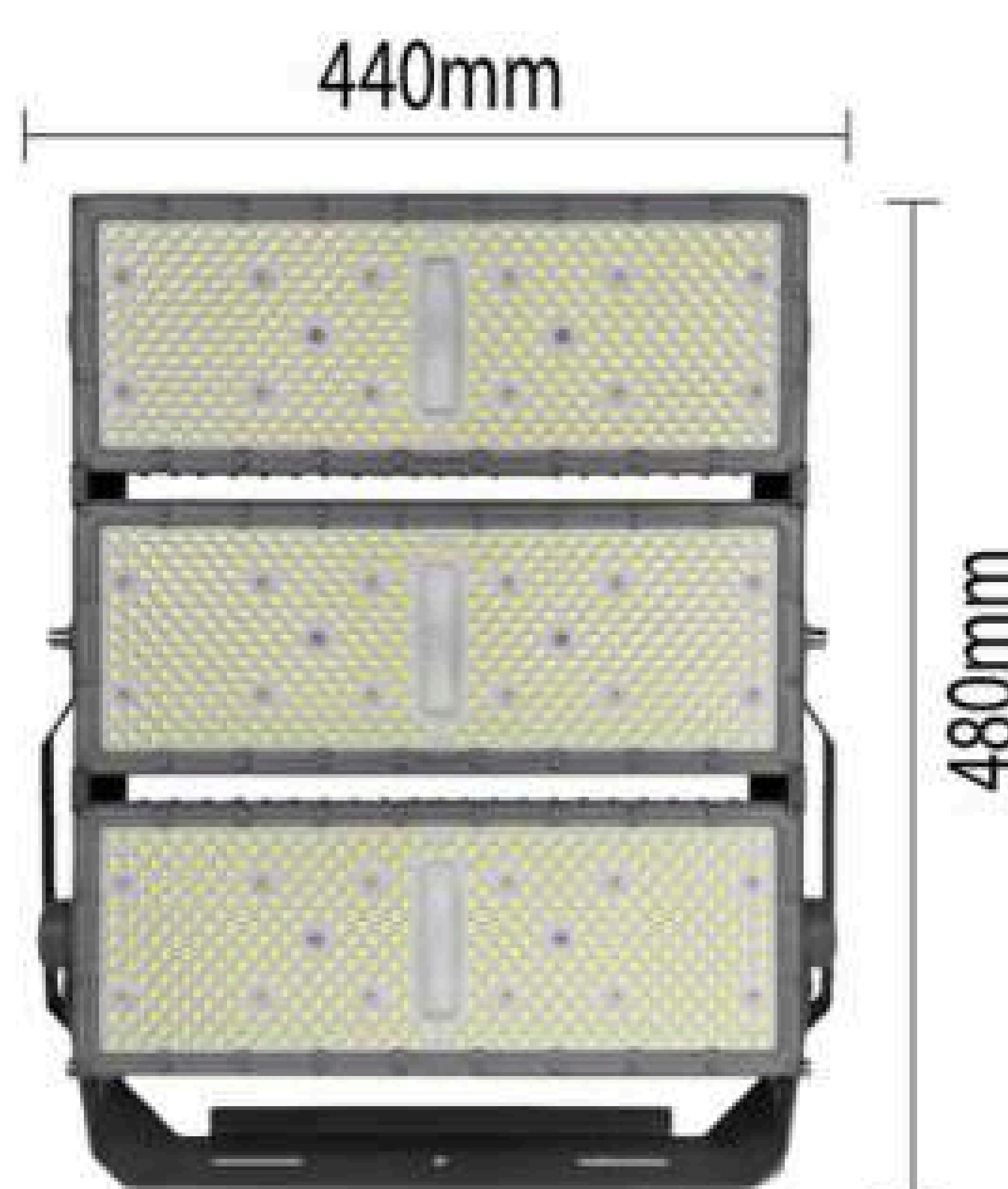
750W PLS-FL750
