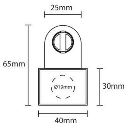
Thick Casing (Single Tube)
