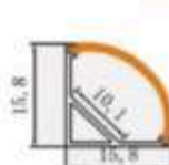
Type C - 16mmx16mm (Surfaced Corner) (Silver / Black)
